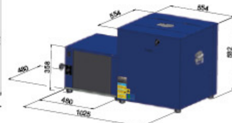
FCOOL 90 1 CV HORIZONTAL
