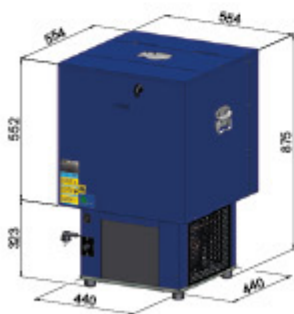
FCOOL 90 1/2 CV VERTICAL
