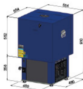
FCOOL 90 1 CV VERTICAL
